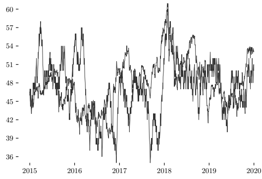
199: Wells Fargo & Coin Tosses
