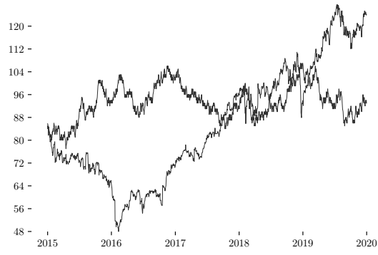
75: American Express & Coin Tosses
