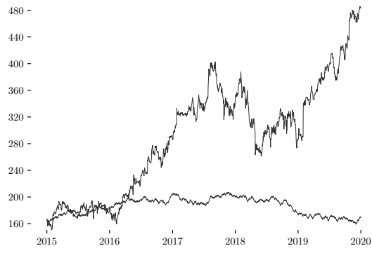
91: Charter Communications & Coin Tosses
